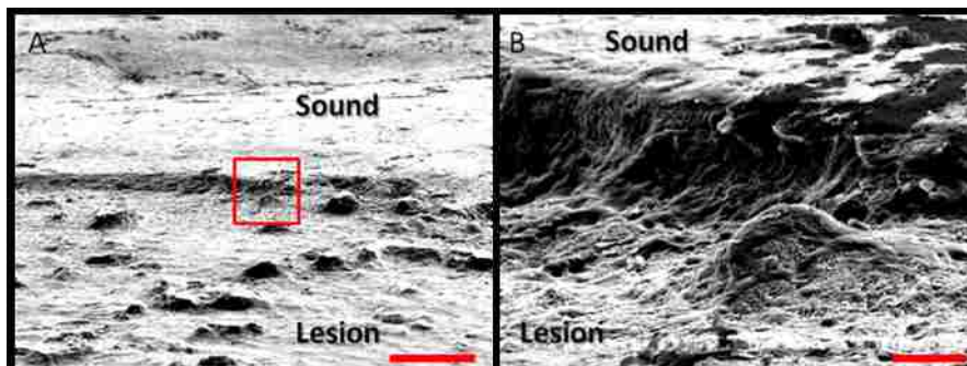
Figure 13: SEM of a specimen after acetic acid demineralization at pH 3 for 1 hour. A) bottom half of the image is the demineralized region. Scale bar is 50 \mu\text{m} . A zoomed in view of the red square box is shown in B. Scale bar is 5 \mu\text{m} . Surface of the eroded region contains pores, which are the result of the loss of mineralization.
