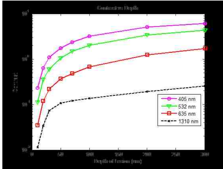
Figure 19: Demineralized enamel contrast of varying depths. MC simulations showed that illumination using 405 nm provided higher contrast than all tested wavelengths. From the simulations, shorter illuminating wavelengths provides higher contrast between sound and demineralized enamel than longer wavelengths.
