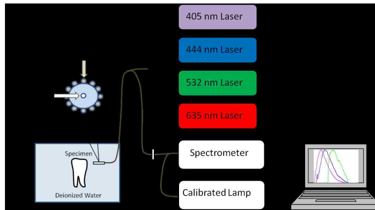
Figure 21: Schematic diagram of the experimental setup. The extracted teeth were held in a chamber filled with water. A custom flexible fiber illuminated the teeth enamel with either a 405 nm, 444nm, 532 nm, or 635 nm laser. The collected fluorescence passed through an in-line optical filter to remove laser light before entering the spectrometer. The spectra were saved on the PC and analyzed offline.
