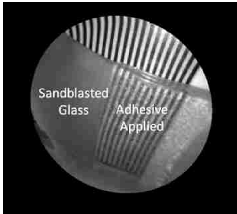
Figure 12: 405 nm image taken of sandblasted glass placed over a test target. The roughened surface scatters the 405 nm light and thus the target is not visible through the sandblasted glass. However, the textured surface was wetted out after application of the transparent viscoelastic pressure sensitive adhesive and thus the target became visible through the glass.
