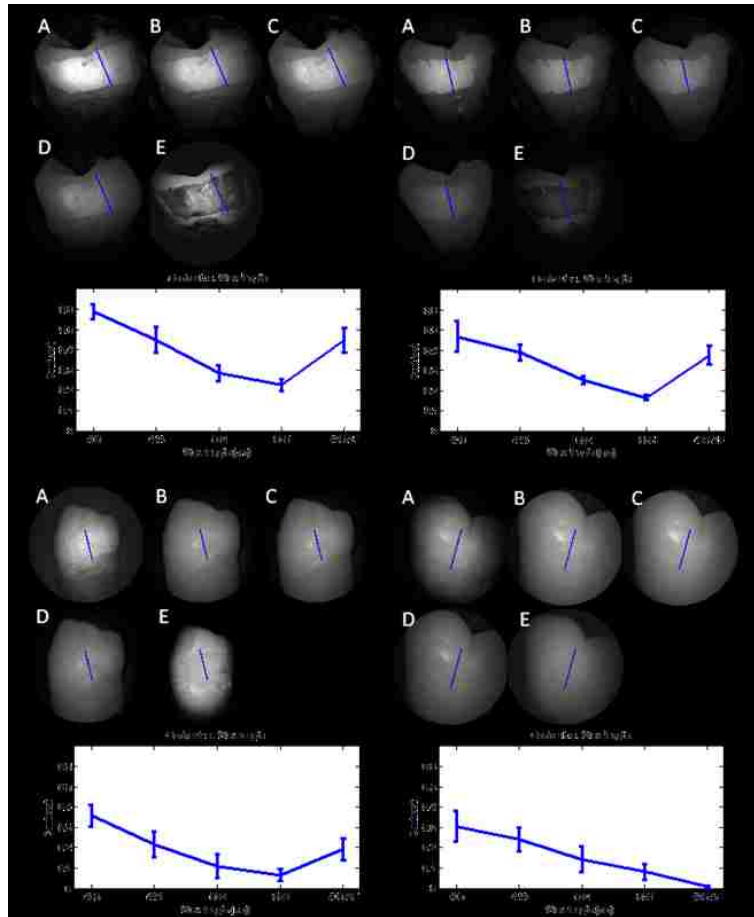
Figure 8: Contrast between erosion and sound enamel for various illuminating wavelengths and acid exposure times. Top left: 6 hour, pH 3 exposure. Top right: 4 hour, pH 3 exposure. Bottom left: 2 hour, pH 3. Bottom right: 1 hour, pH 3. For all four panes, A) 405 nm reflected image, B) 444 nm reflected image, C) 532 nm reflected image, D) 635 nm reflected image, and E) 405 nm illuminated autofluorescence image. Mean and standard deviation of measured contrast for each imaging modality are shown in the plots. Blue line in each image indicates location where contrast was measured.
